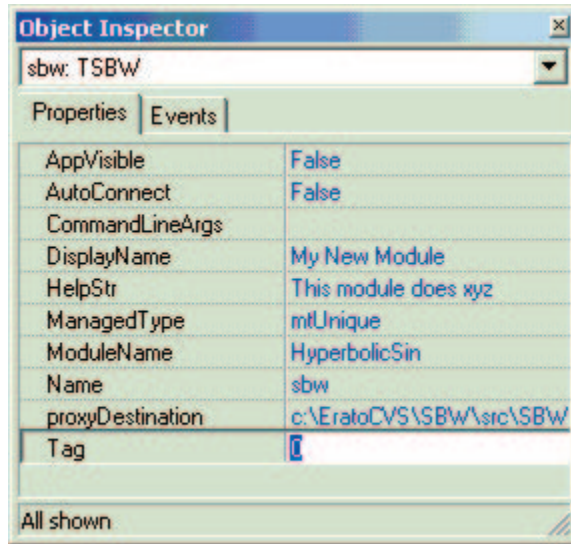
Figure 2: Properties List for TSBW Component
